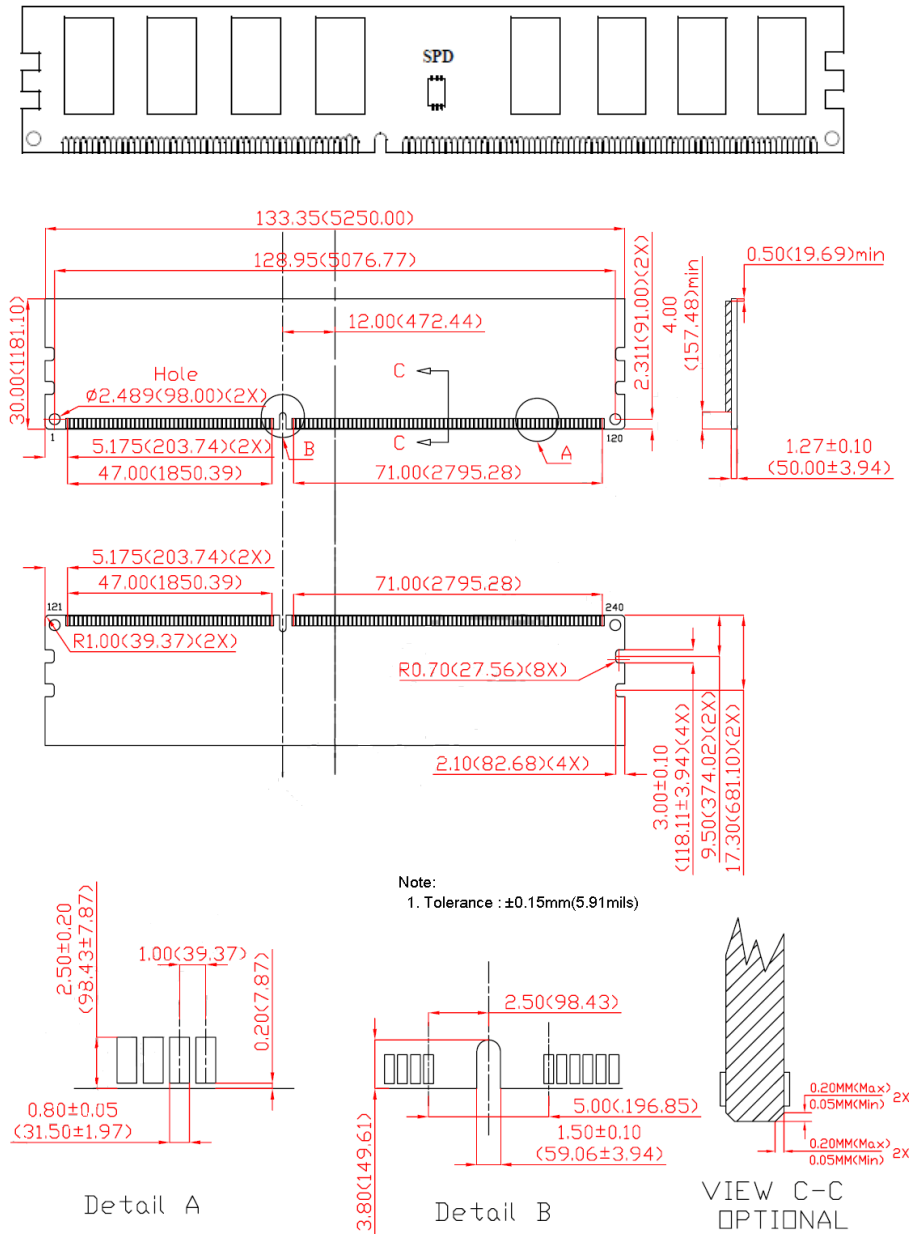
Figure 1 - Package Dimensions
